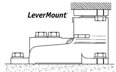
Stainless steel load foot Acc.35901
