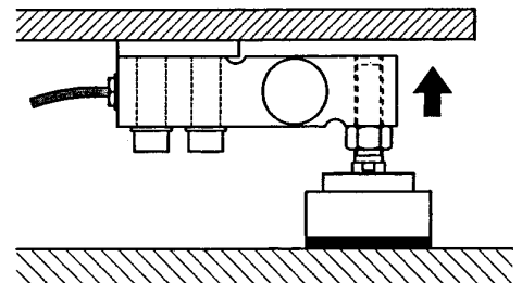
Stainless steel load foot Acc.35901
